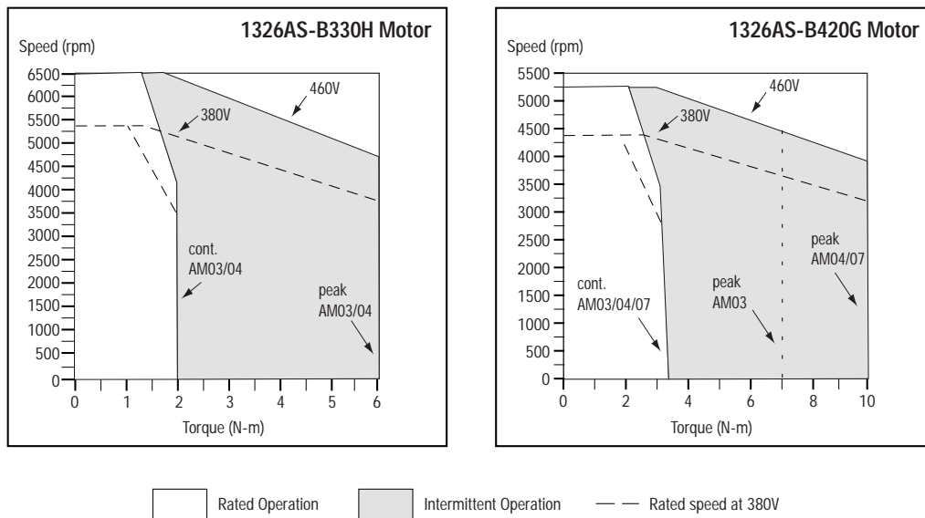
Figure 3 1326AS-B330H and 1326AS-B420G Speed-Torque Curves
