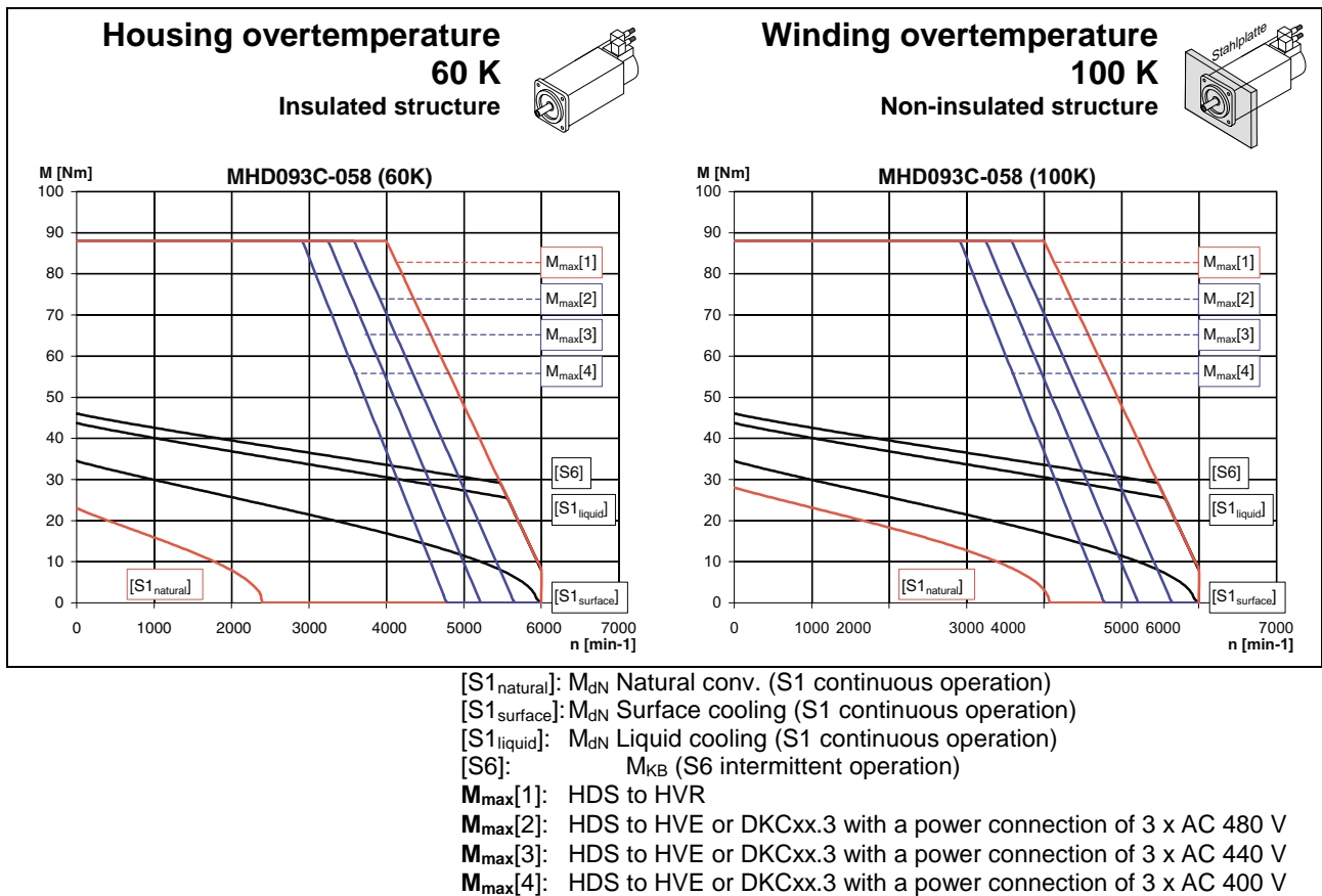
Fig. 9-14: Characteristic curves
