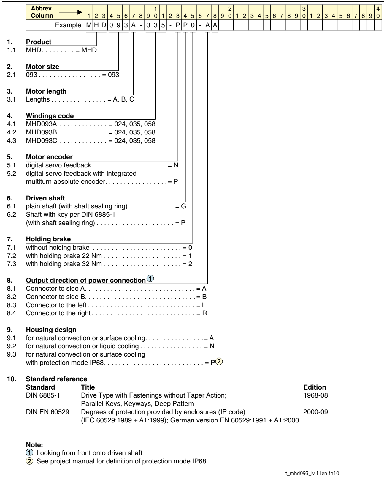
Fig. 9-12: type code MHD093
