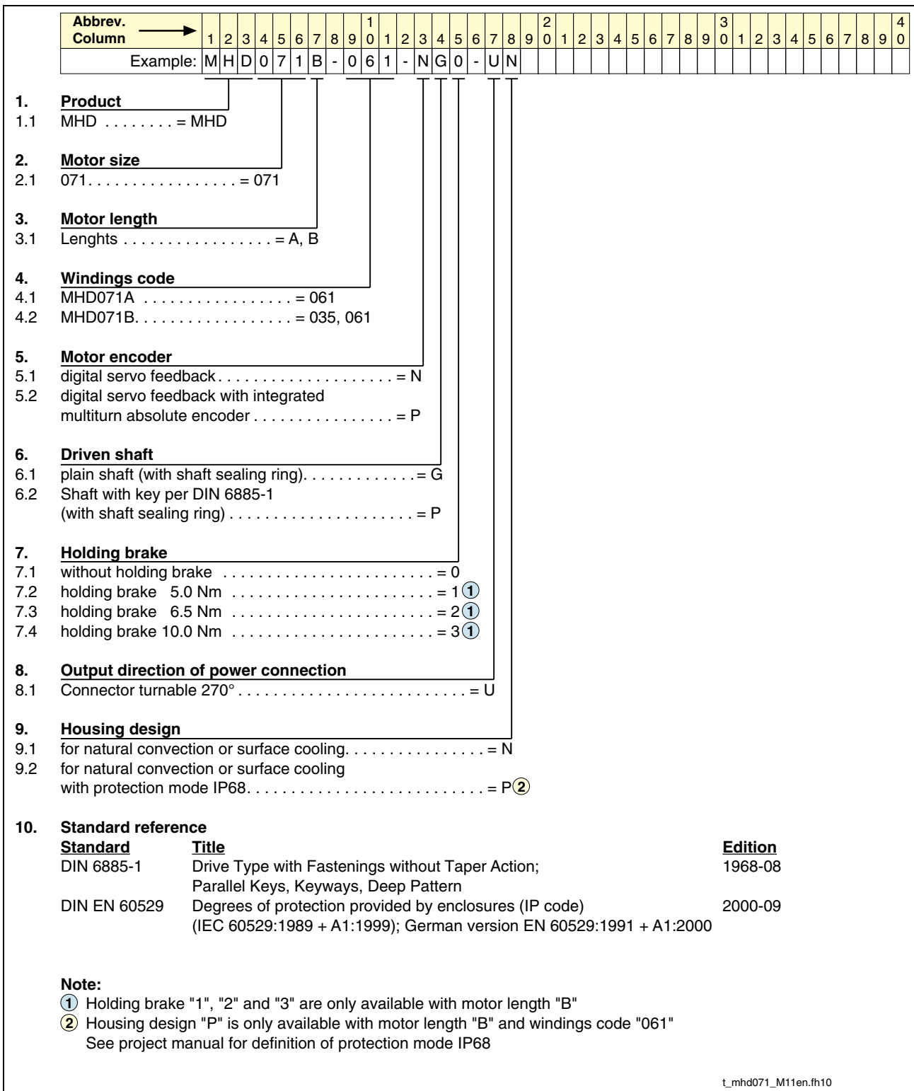
Fig. 7-5: MDH071 type code
