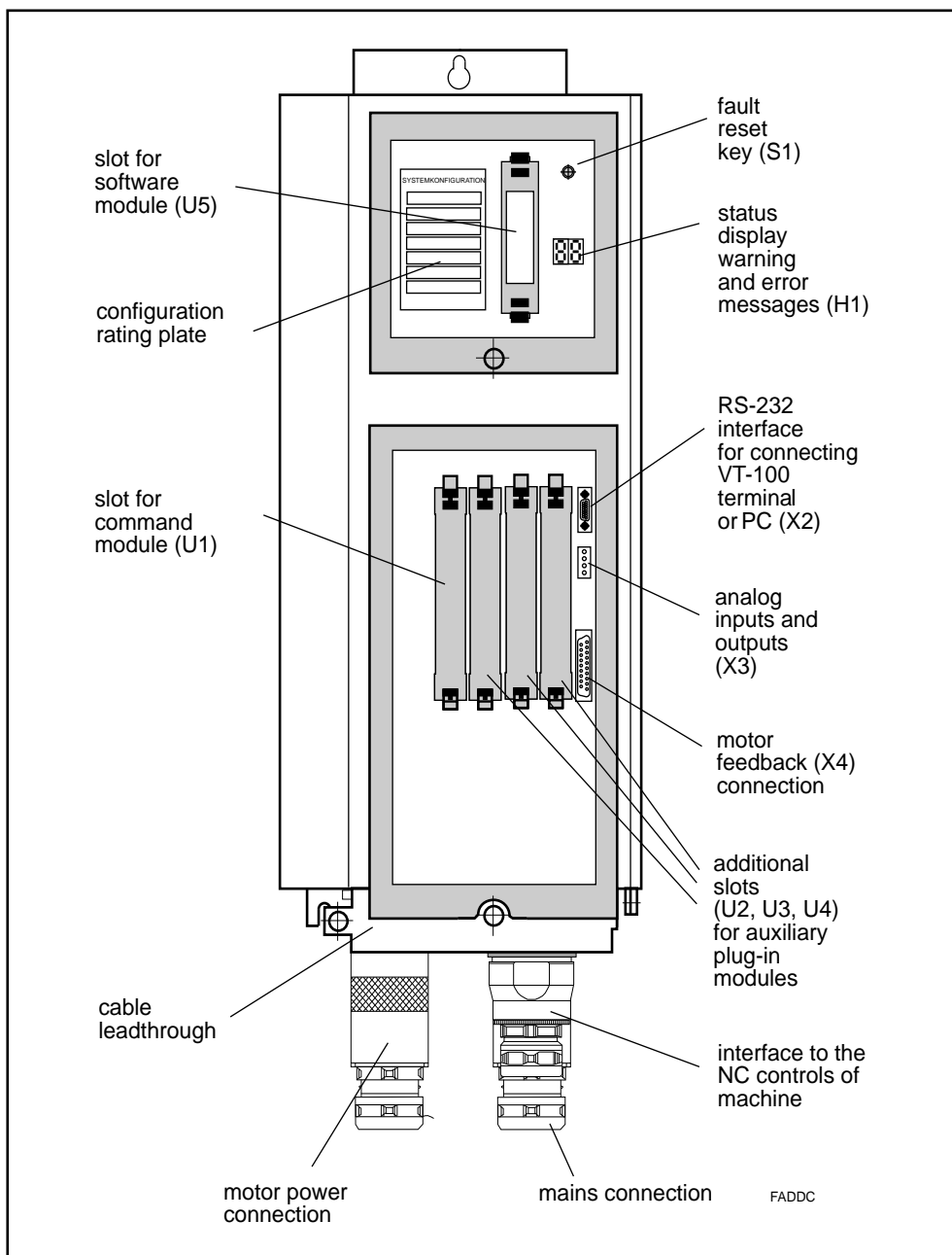
Fig. 4.2: Front view of DDC 1.2-N
