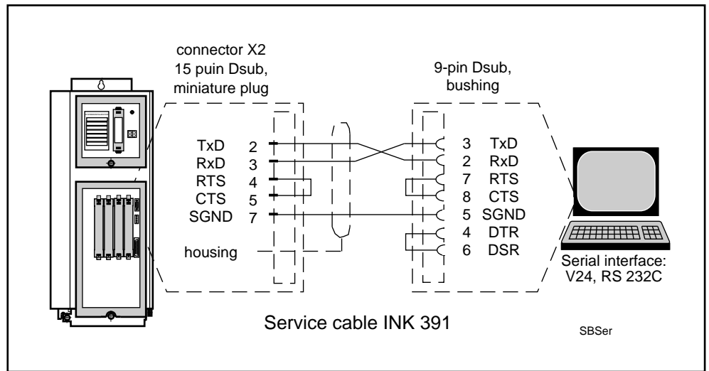
Fig. 3.19: RS 232 interface
